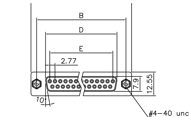
#4-40 unc screwlock installed
