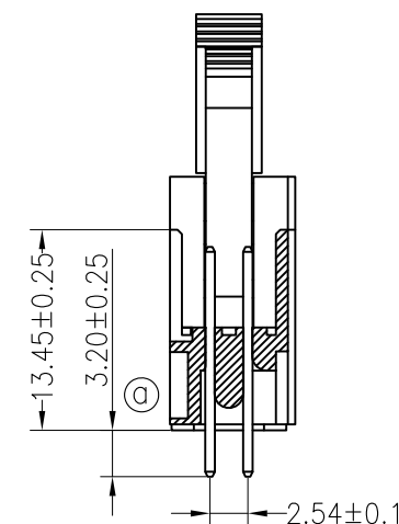
Short Latch
